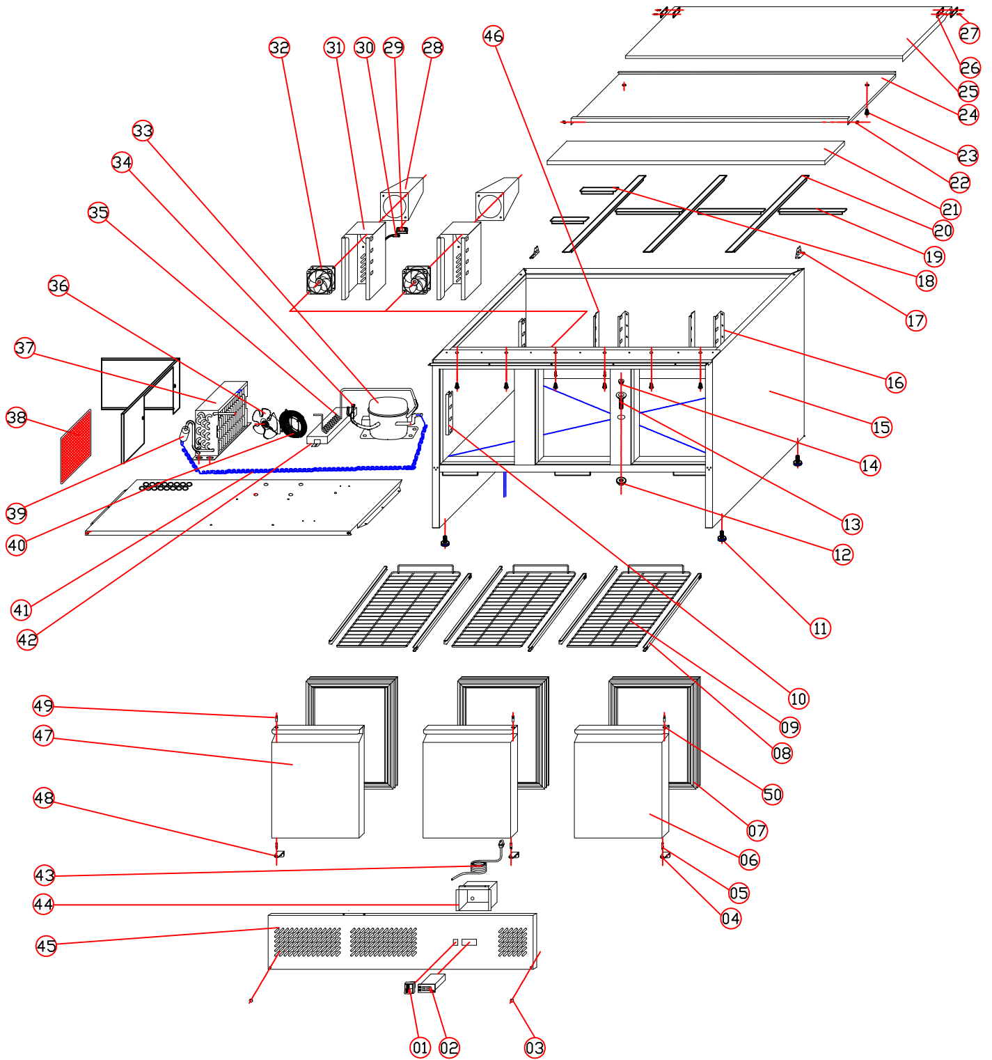
EXPLODED VIEW OF S903 STD
